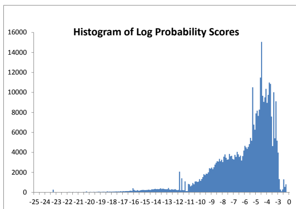
Figure 2: Histogram of log probability scores obtained from Web N-gram service
